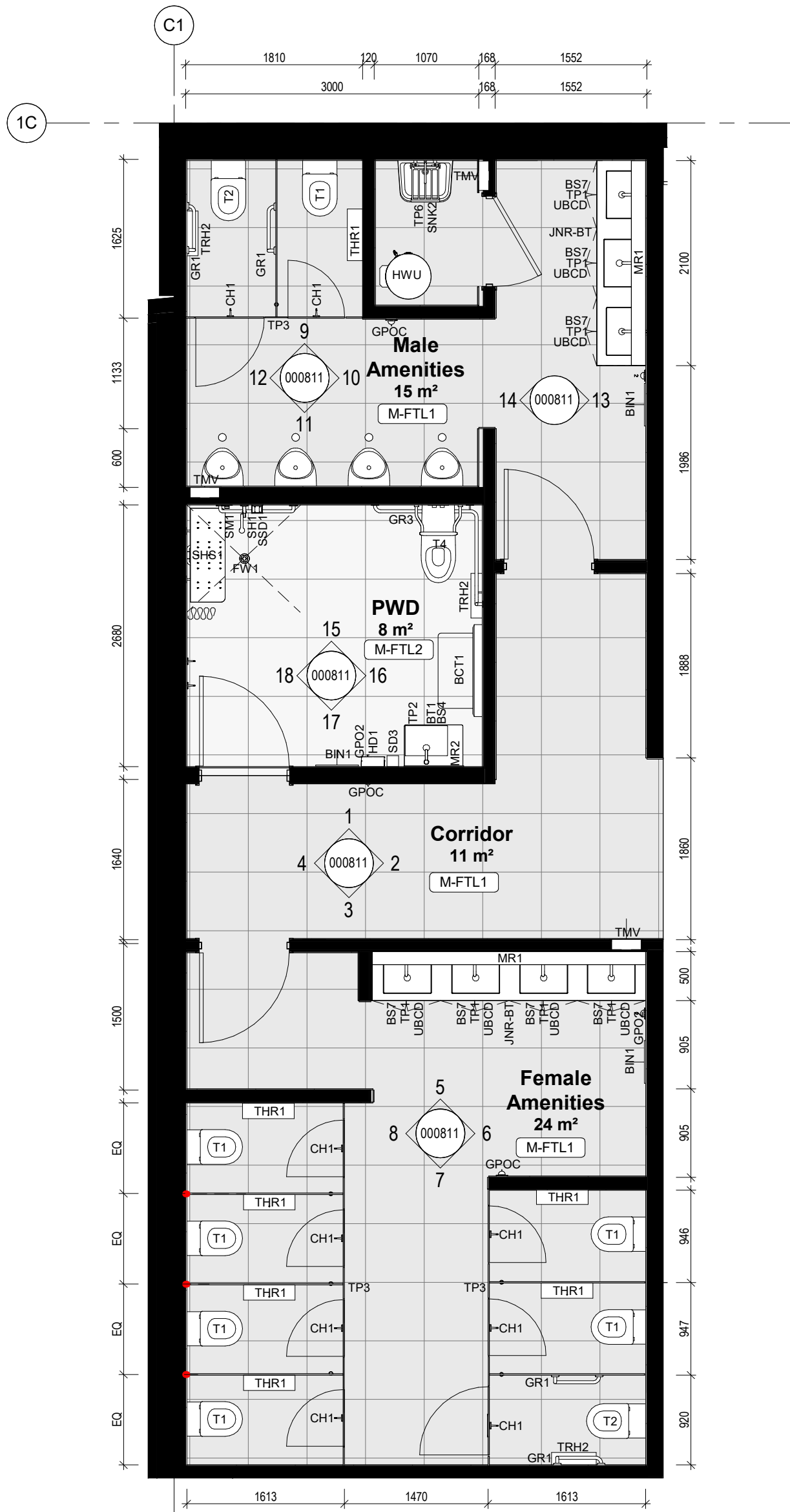
2 WET AREA PLAN - GAME OVER 1 : 50
